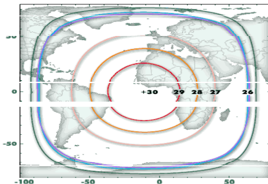
Ekspress 3A Ku Band Coverage
