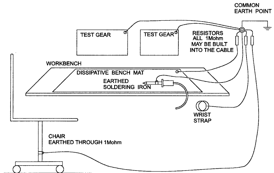
Fig 1. STATIC SAFE WORK AREA
